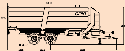
ROLLFEED 6218
