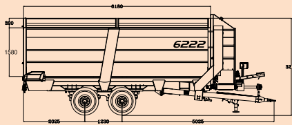
ROLLFEED 6222
